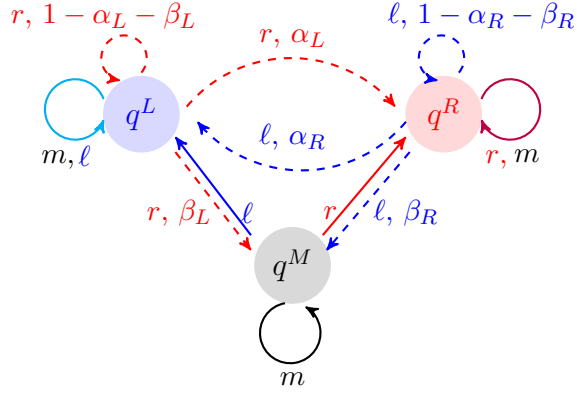
Figure 1: Optimal 3-state automaton FA_3(\alpha_R, \beta_R, \alpha_L, \beta_L)
